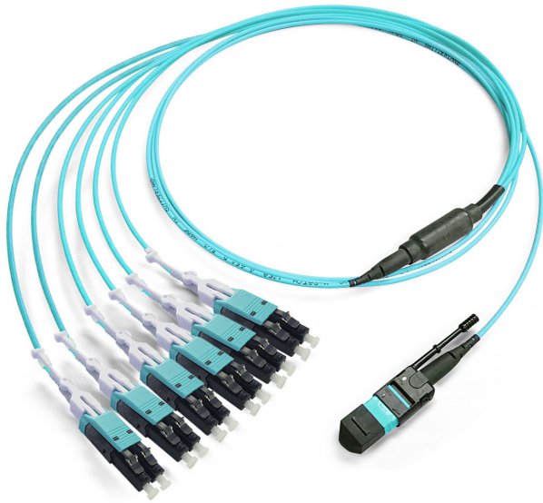
Cable DCS fanout MTP-LCDU, 12 fibras OM3
